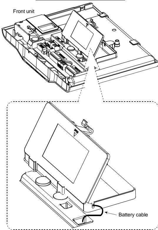
Figure 10. Battery Replacement
